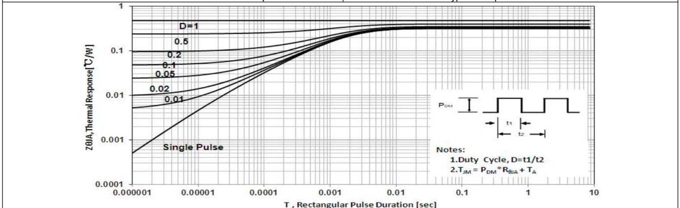
Maximum Effective Thermal Impedance, Junction to Case
