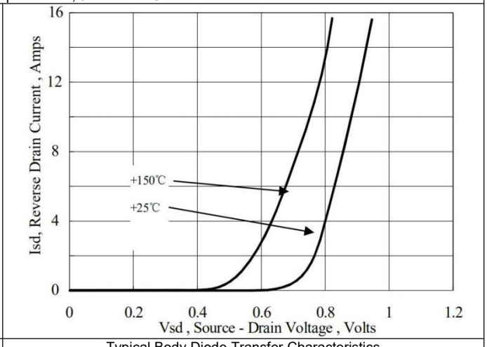
Typical Body Diode Transfer Characteristics
