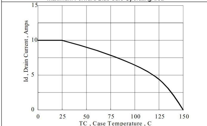
Maximum Continuous Drain Current vs Case Temperature
