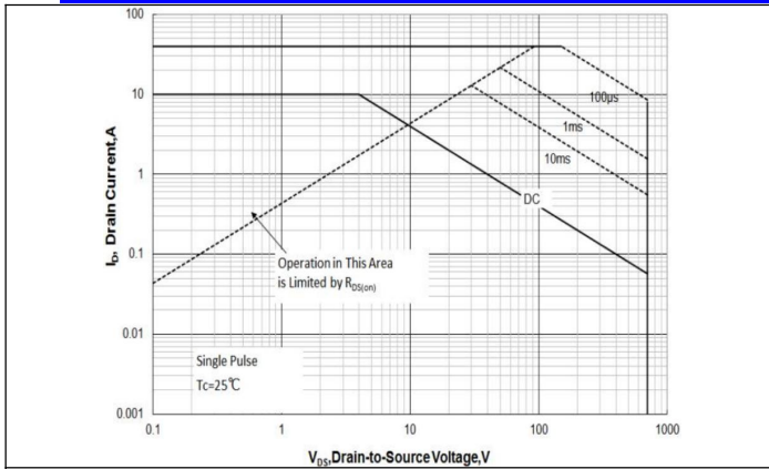
Maximum Forward Bias Safe Operating Area
