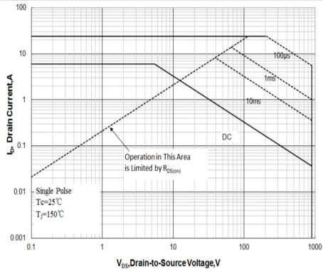
Maximum Forward Bias Safe Operating Area
