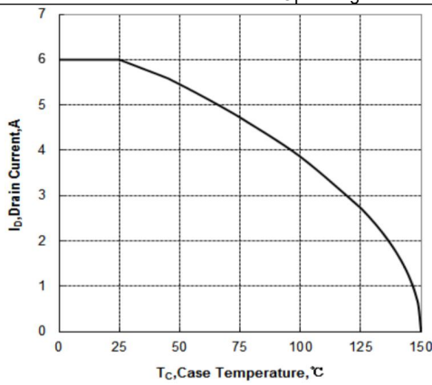
Maximum Continuous Drain Current vs Case Temperature
