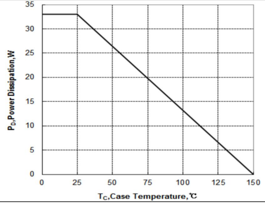
Maximum Power Dissipation vs Case Temperature
