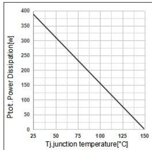
Fig4. Power Dissipation of temperature characteristic
