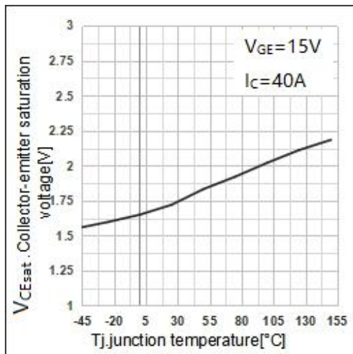
Fig3. Collector-emitter saturation voltage
