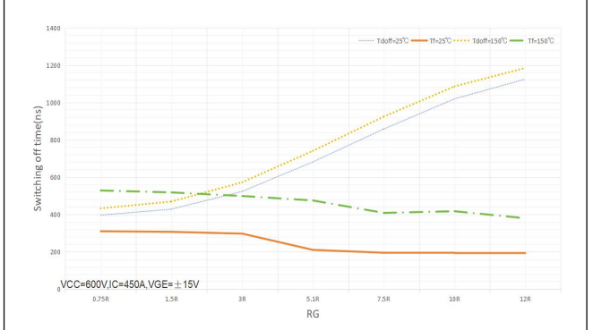
Switching off time vs. RG
