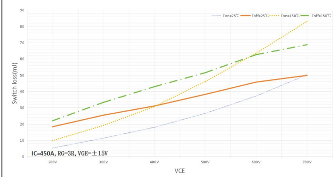
Switch loss vs. VCE
