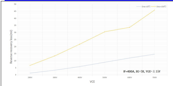
Diode directional recovery loss vs. VCE
