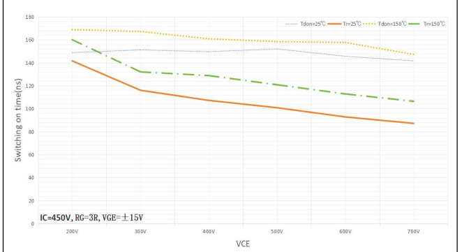
Switching on time vs. VCE
