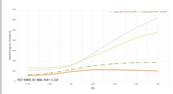
Switching on time vs. RG
