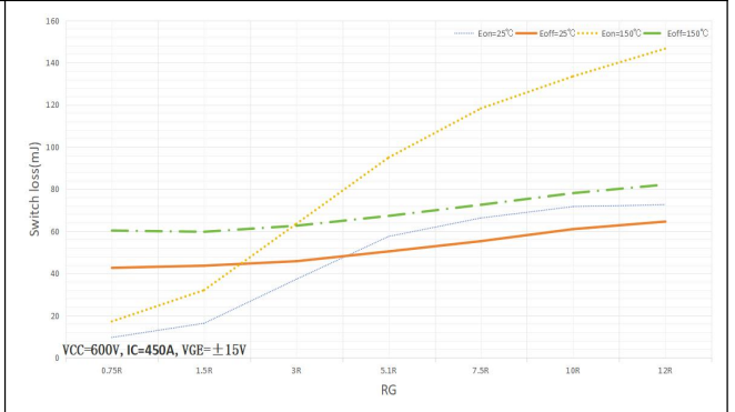
Switch loss vs. RG
