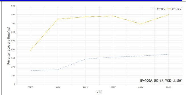
Diode reverse recovery time vs. VCE
