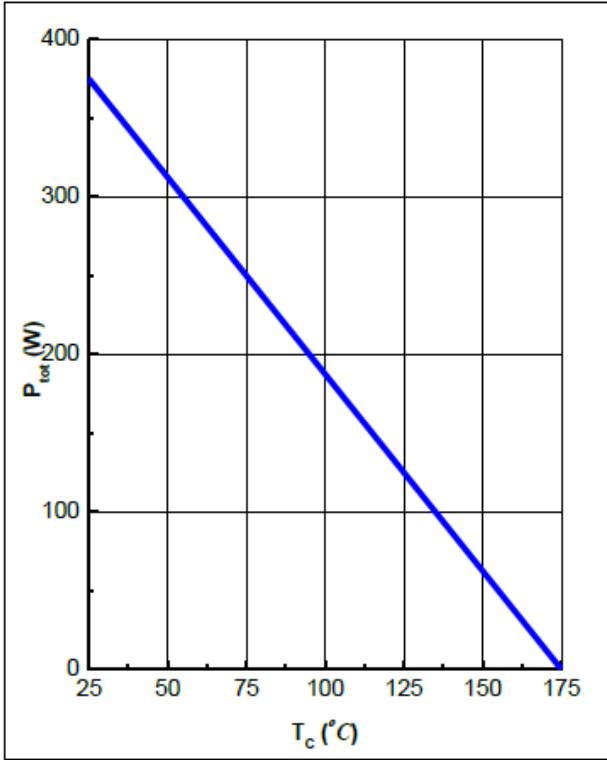
Figure 3. Power Derating
