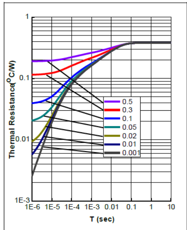
Figure 6. Transient Thermal Impedance
