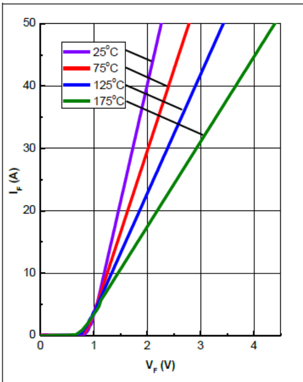
Figure 1. Forward Characteristics
