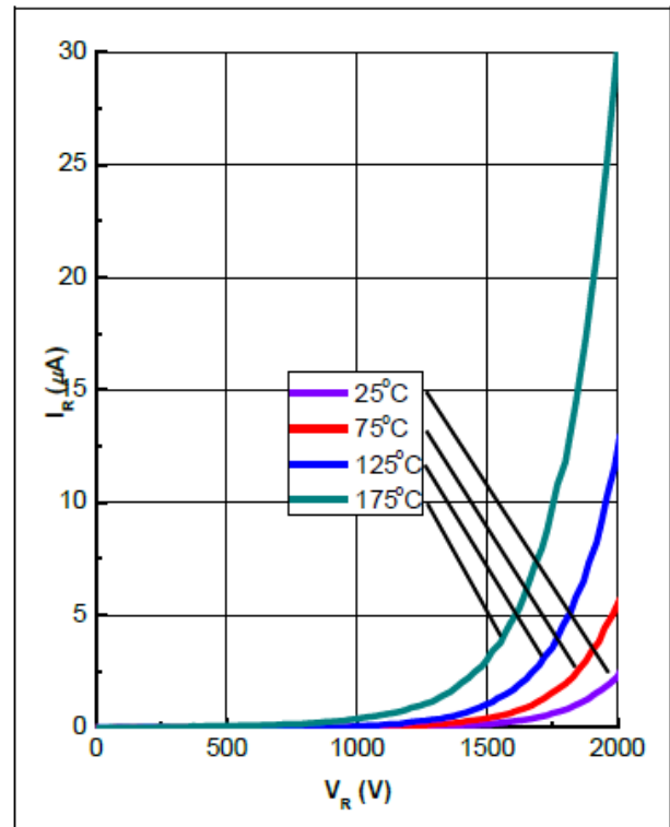
Figure 2. Reverse Characteristics
