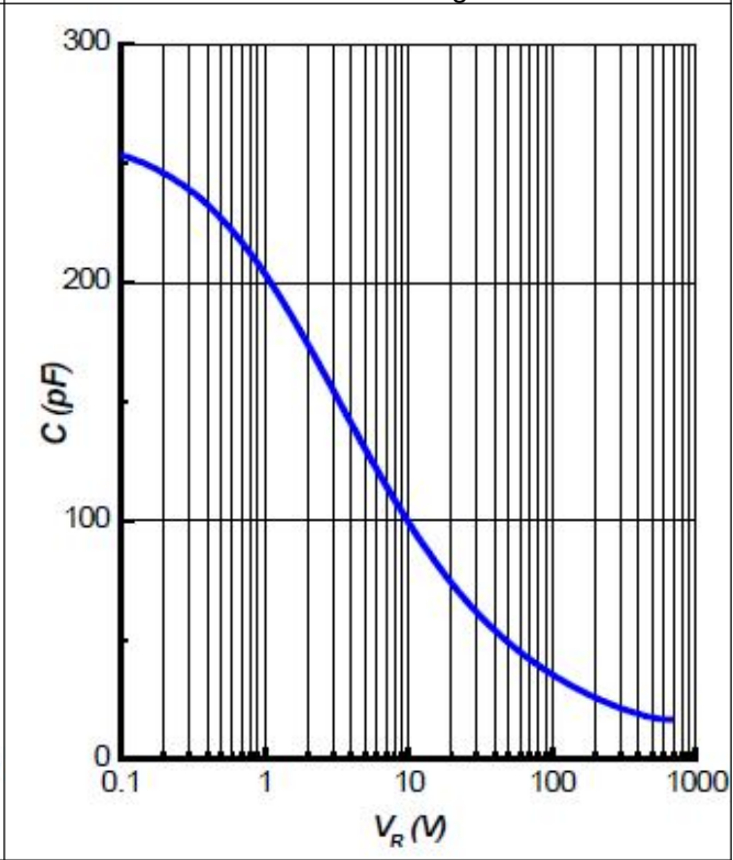
Total Capacitive Charge vs. Reverse Voltage
