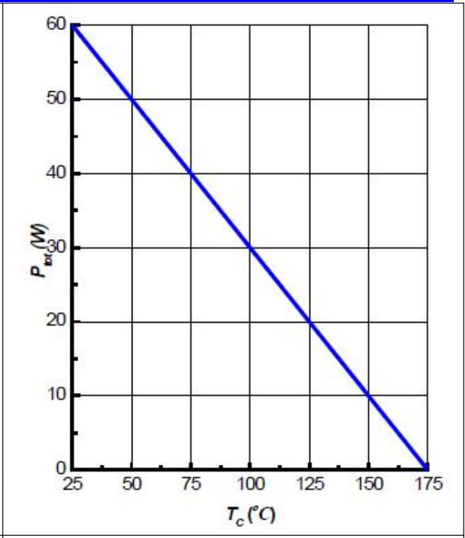
Power Derating
