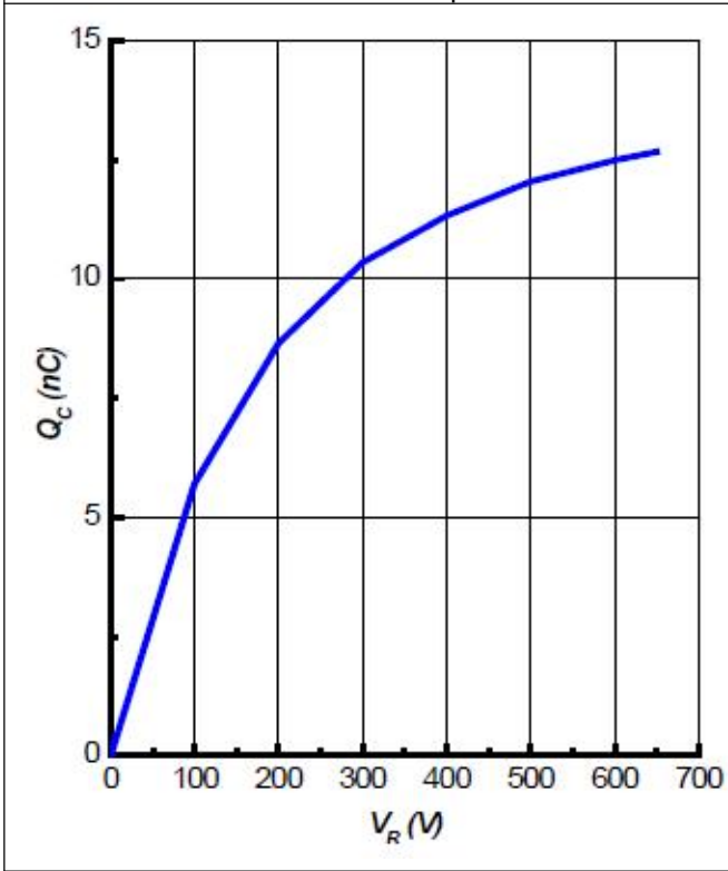
Total Capacitance Charge vs. Reverse Voltage
