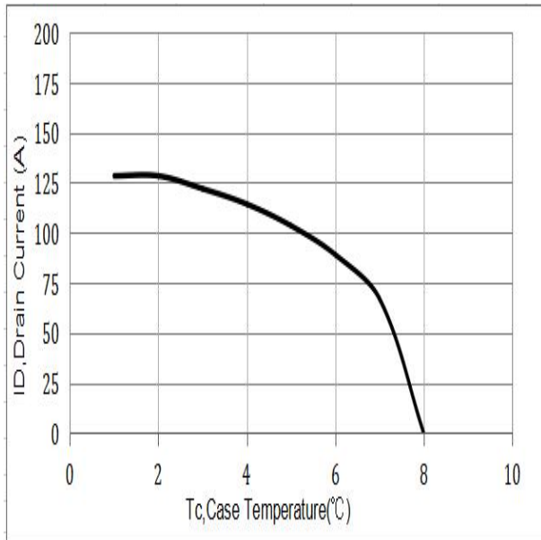
Figure 8. Power De-rating
