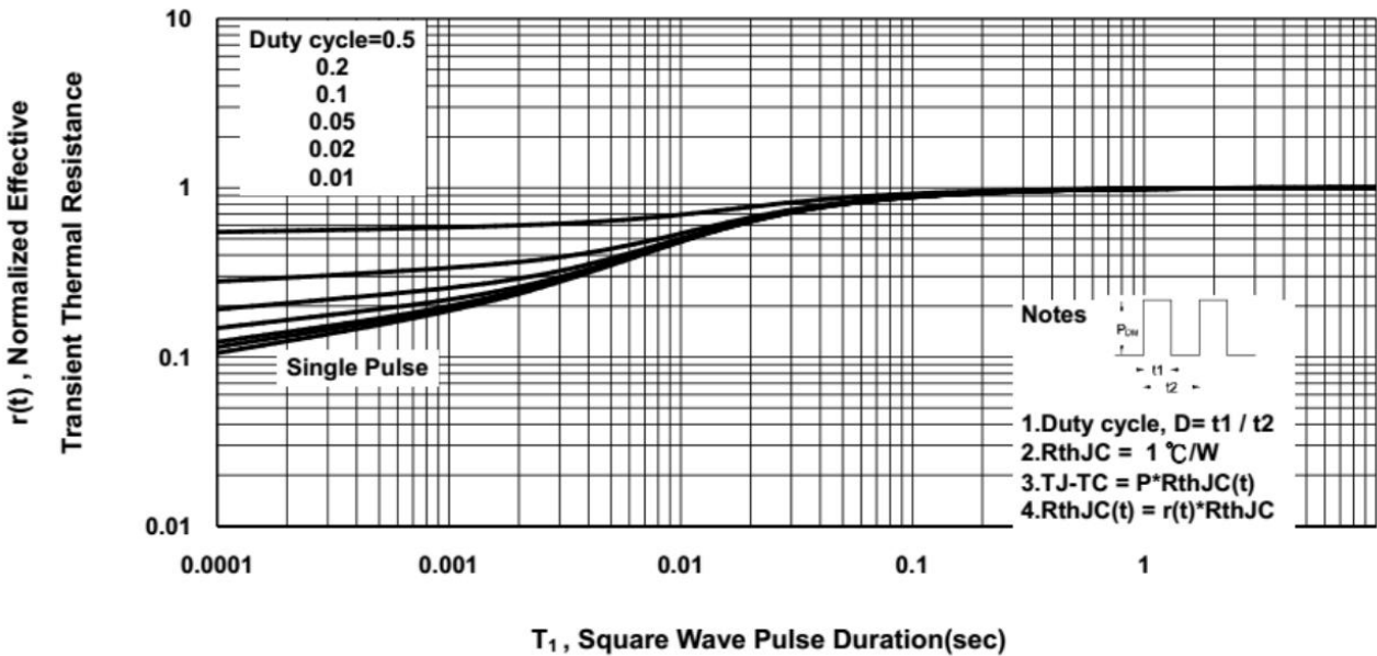
Fig 11 T1 , Transient Thermal Response Curve
