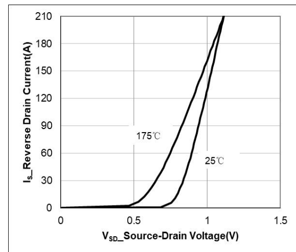
Figure 6 V_{SD\_Source-Drain\ Diode\ forward}
