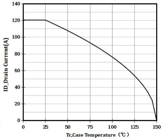
Figure 8 Current De-rating
