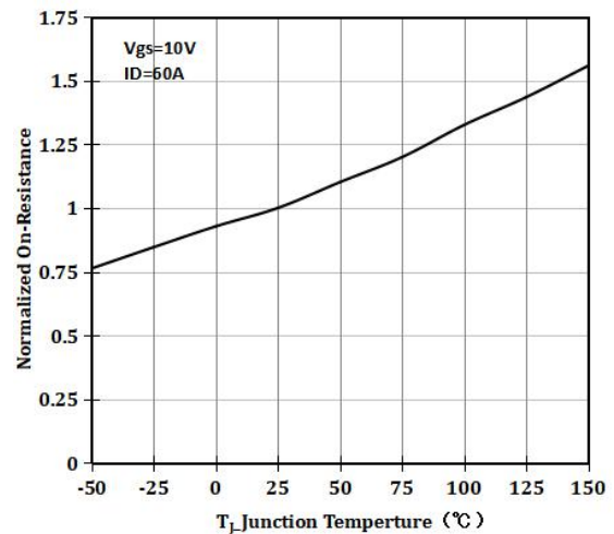
Figure 6 Rds(on)-Junction Temperature
