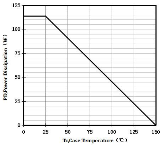
Figure 7 Power De-rating
