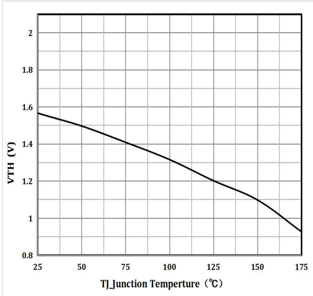
Figure 5 Threshold vs Temperature
