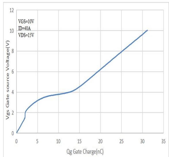
Figure 4 Gate Charge
