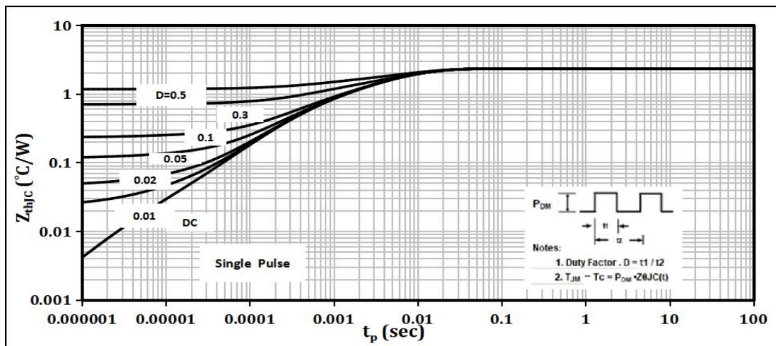
Figure 7 Normalized Maximum Transient Thermal Impedance
