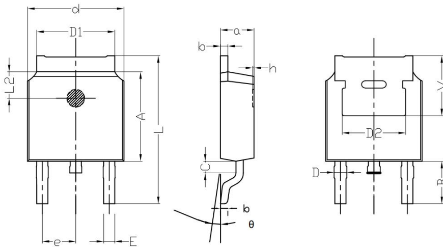
TO-252B PACKAGE OUTLINE DIMENSIONS
