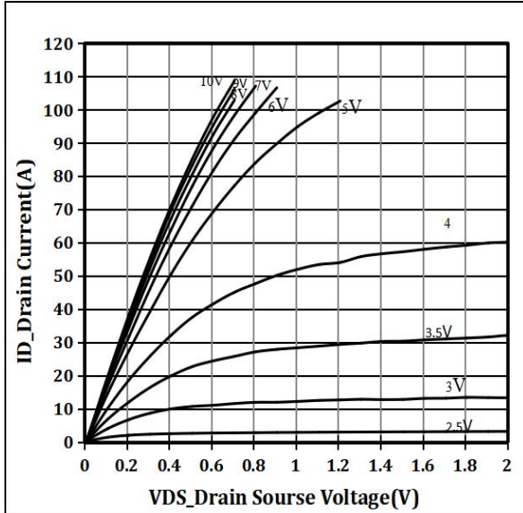
Figure 1 Output Characteristics
