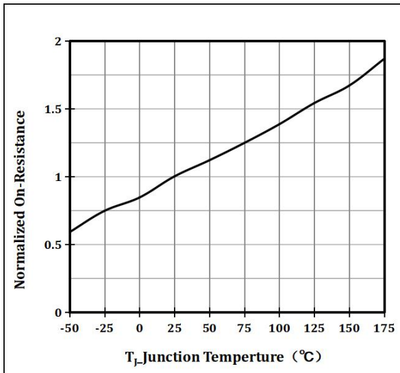
Figure 3 R_{DS(ON)} - Junction Temperature
