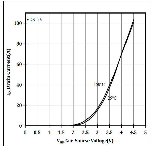
Figure 2 Transfer Characteristics
